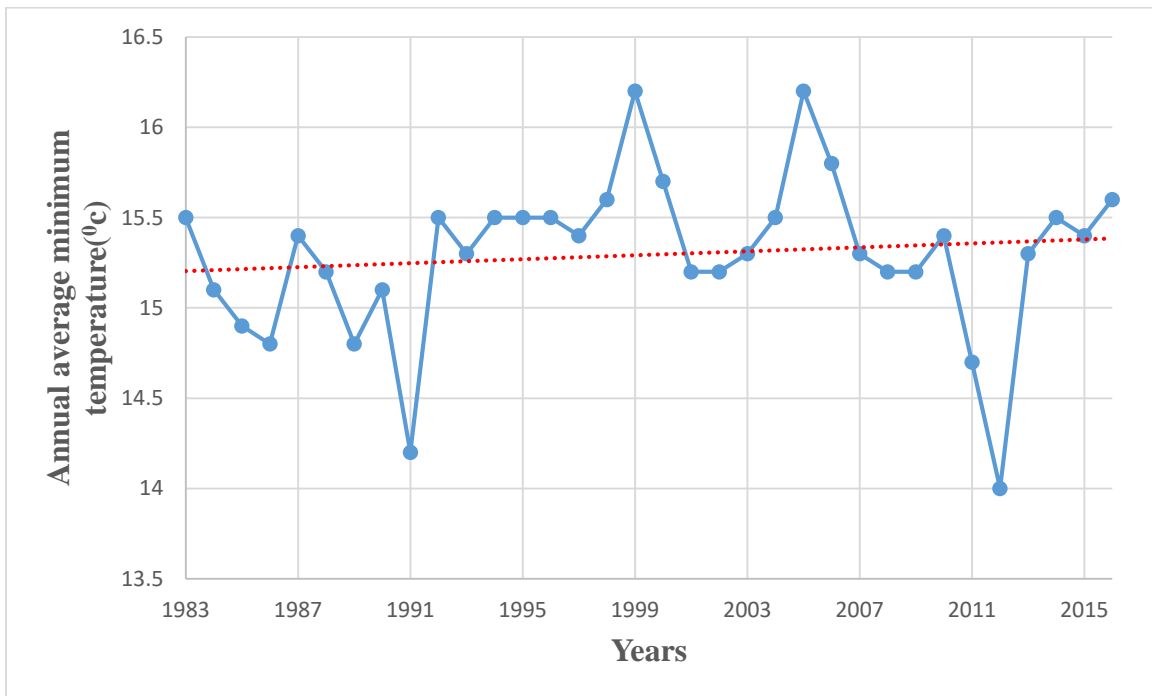
Figure 18: Mann Kendal Trend Analysis of Annual maximum Temperature for Bugesera District over Eastern province from 1983 to 2016.
