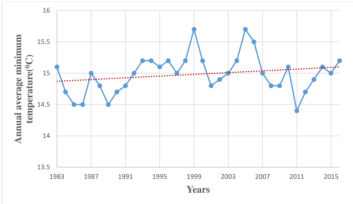
Figure 17: Mann Kendal Trend Analysis of Annual Average Minimum Temperature for Nyagatare District over Eastern province from 1983 to 2016.
