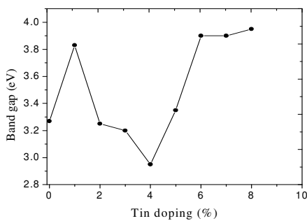
Figure 3.6: Variation of band gap with tin doping concentration. The lowest band gap was obtained at 4% tin doping
