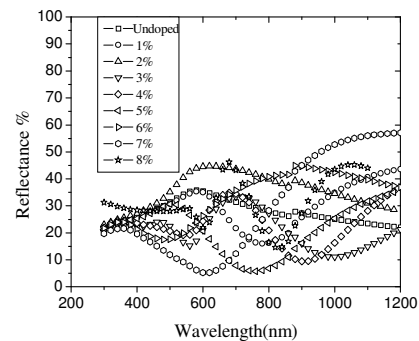
Figure 3.2: Optical reflectance of tin doped zinc oxide
