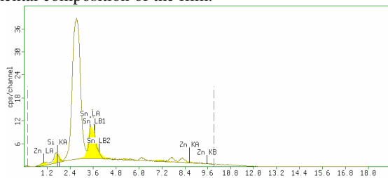
Figure 3.9: XRF spectrum of ZnO:Sn thin film with 4% Sn doping concentration
