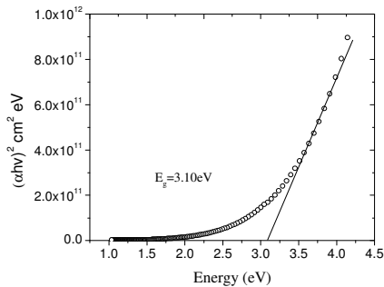
Figure 3.5: Extrapolation of the linear part of (\alpha hv)^2 against energy (eV) for tin doped zinc oxide. The band gap energy was obtained was 3.10 eV for 3% tin concentration
