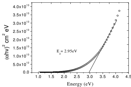
Figure 3.4: Extrapolation of the linear part of (\alpha hv)^2 against energy (eV) for tin doped zinc oxide. The band gap energy was obtained was 2.95 eV for 4% tin concentration
