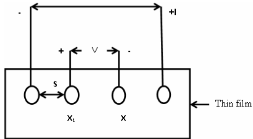
Figure 2.0: The four point probe linear set up
