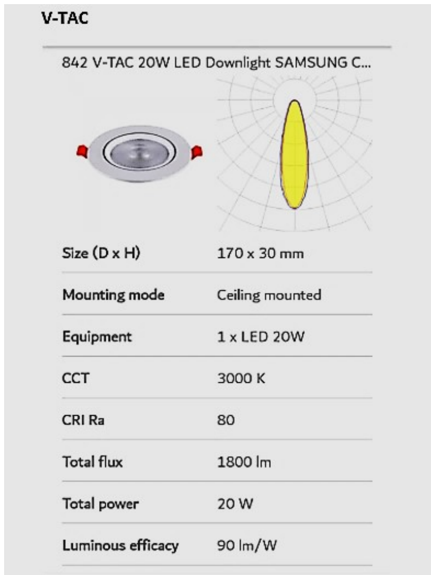
Figure 3.1 Lighting and Mounting Properties for Washroom
