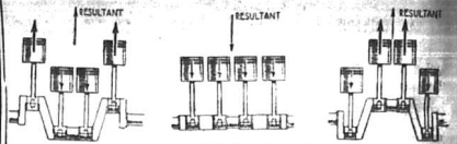
Three diagrams which show the forces exerted by the rapidly moving pistons of a four-cylinder engine. As a result the power unit tends to vibrate up and down.
