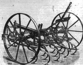
THE IPOWICH STEEL CULTIVATOR 17 TINE MODEL.
