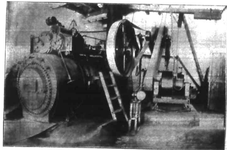
THE ORIGINAL PLANT WHICH HAS PROVIDED LIGHT FOR MOMBASA SINCE 1905.
