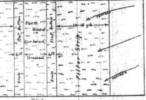
Showing water disposal from terraces using a "filter strip" of grass and grassed drains on either side of a grassed and cambered farm road.
