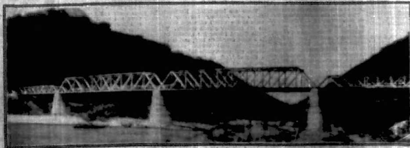
The great Ruaha Bridge of 4 spans with a total length of 600 feet on the Kilosa-Hakara Road. Photo: C. V. Stevenson.
