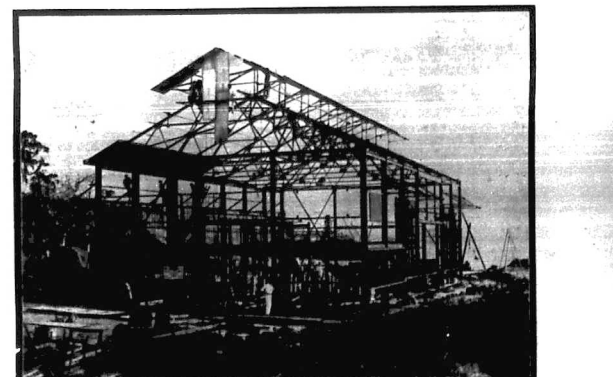
NEW ELECTRIC LIGHT AND POWER STATION (Shimani-Mombasa Island) Showing progress made in the erection of the new works.
