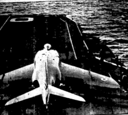
Below is a new fighter-bomber for the Royal Navy - the Vickers V.I.E. It has a new flap system operated by high-pressure air fed through the rear of the wings as a sheet. The aircraft is seen while on catapult and deck landing trials on the aircraft-carrier Eagle of Southern England.
