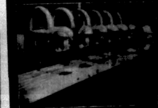
A special setup in the factory of the Union Special Machine Co. for the drilling of heavy industrial machine tools. Note the wide bench provided by the special Taucu Drill Press. 17-inch Taucu Drill Presses, similar to those shown in this illustration are used extensively by British engineering works.
