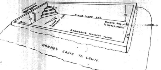
A diagram of the pool which should be fitted on a slope. This allows for varying depths of water and drainage of the bath by merely turning a tap.
