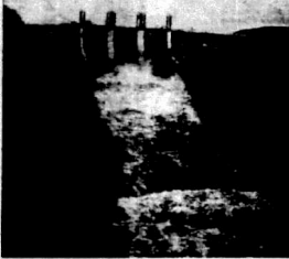
The spillway gates discharging water downstream in the Tana River. The electrically operated gates are raised between the columns and are designed to allow for a flow of 100,000 cubic feet of water per second, which is a third greater than the highest flow of water recorded during the 1962 season.
