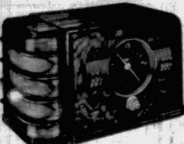
ZENITH 7000 —A Super Table Top Radio—7-tube super-heterodyne with Transcontinental Automatic Tip-Touch Tuning receiver American, foreign broadcasts, police, amateur, aviation, ships; 8-inch speaker; Radiorgan; 23 inches wide, genuine walnut finish. No. 700.
