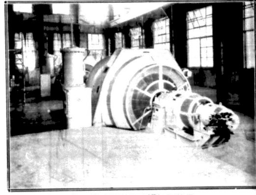
A corner of the power house showing the 2,000 h.p. generating sets.
