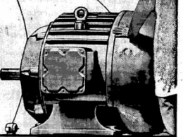
Cooling air stream is drawn into motor, and guided by deflectors, which are also water proofed. For maximum efficiency, the cooling air is drawn through openings in the frame casting.
