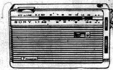
SONY TR-716 2-band portable with dial lamp and fine tuning control. Gives excellent performance with amazingly high sensitivity and selectivity. SONY TR-716B (MW; SW 77-25m); SONY TR-716Y (MW; SW 50-16m). Uses two economical flashlight batteries (size C).
