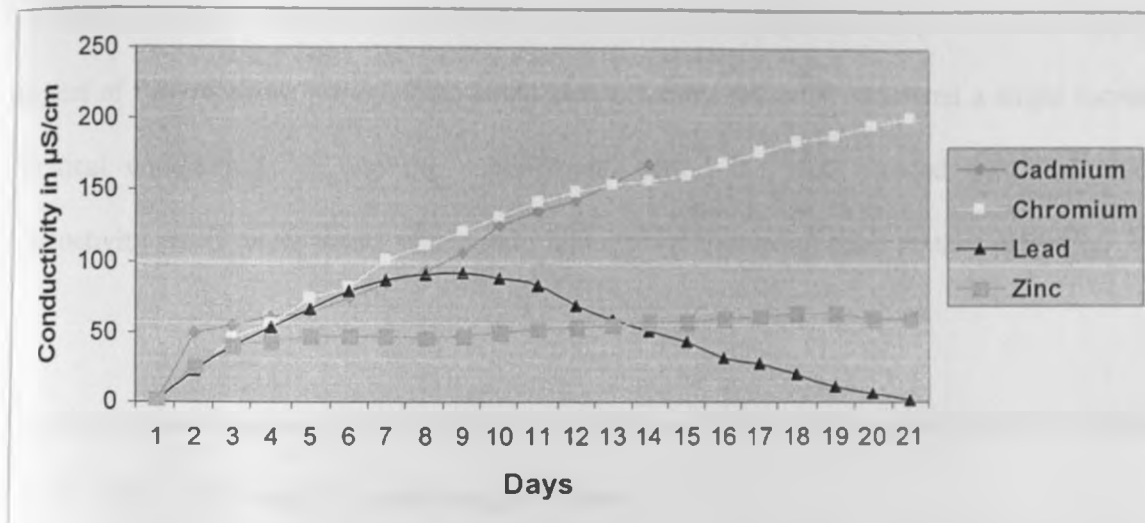
Figure 4.28: Comparison of mean electrical conductivity in \mu\text{S/cm} of heavy metals in 20ppm metal solutions containing variety UP-D.
