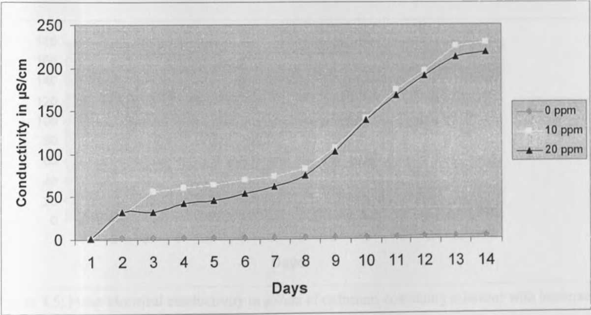
Figure 4.4: Mean electrical conductivity in \mu\text{S/cm} of cadmium-containing solutions with immersed UP-C variety.
