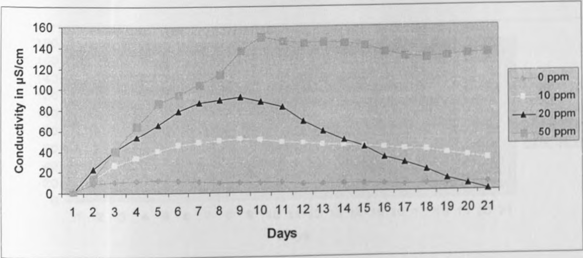
Figure 4.23: Mean electrical conductivity in \mu\text{S/cm} of lead-containing solutions with immersed UP-D variety.
