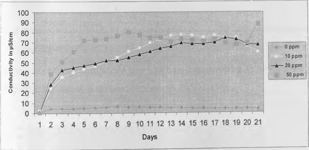
Figure 4.15: Mean electrical conductivity in \mu S/cm of zinc-containing solutions with immersed UP-B variety.
