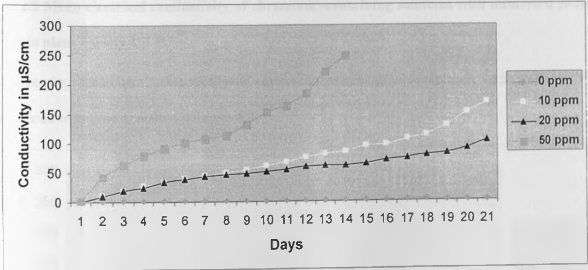
Figure 4.8: Mean electrical conductivity in \mu\text{S/cm} of chromium-containing solutions with immersed UP-A variety.
