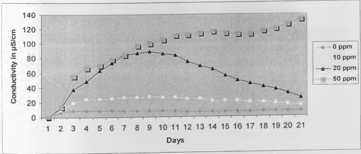
Figure 4.22: Mean electrical conductivity in \mu S/cm of lead-containing solutions with UP-C variety.
