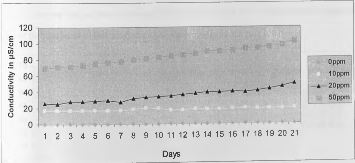
Figure 4.19: Mean electrical conductivity in \mu\text{S/cm} of control solutions of lead without plant varieties.
