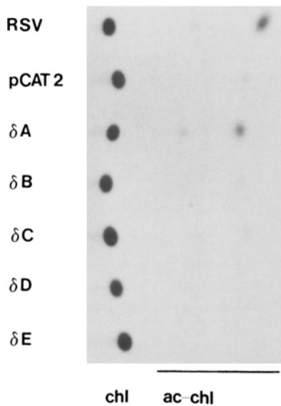
FIGURE 1. Localization of the TCR- \delta enhancer by transfection of CAT vectors into the Peer cell line. (A) Restriction map of the 3' part of the TCR- \delta locus and definition of the DNA fragments inserted in CAT expression vectors. (B) Demonstration of the presence of a transcriptional positive regulatory sequence inside the \delta A DNA fragment by transient transfection assays in the Peer cell line. The transfected cell extract was assayed for its ability to convert chloramphenicol (chl) to the acetylated form (ac-chl). The DNA fragment inserted in the polylinker located 3' to the CAT gene in the expression vector is indicated beside each lane. RSV-CAT (RSV) and pCAT2 constructions (see Materials and Methods) are used as positive and negative controls, respectively. A clear enhancement is observed in lane \alpha A , but not in lanes \delta B , \delta C , and \delta E . All data shown in this panel were obtained in the same series of transfection experiments. (C) Study of the transcriptional activity associated with subfragments from \delta A . \delta A and \delta A.1 fragments were cloned in opposite orientations in the CAT vector, showing that transcriptional enhancement is independent of the orientation in which the enhancer is cloned. Note that less extract was changed in the \delta A.11 lane than in other lanes. In this lane, percentage of acetylation is 45%, compared with 4% in the negative control pCAT2 lane. For details, see text.
