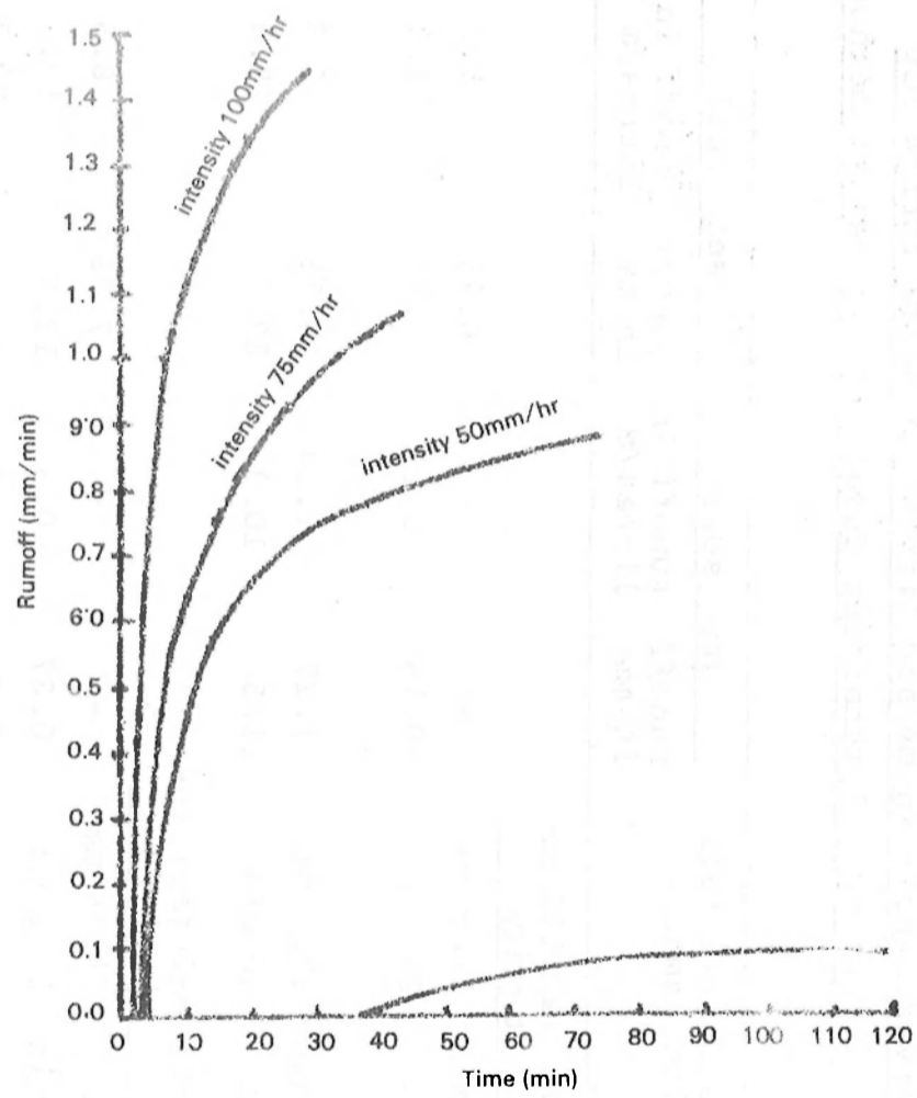
FIG. 9 (b): Runoff time graph for varying rainfall intensity - Katurmani dry soil
