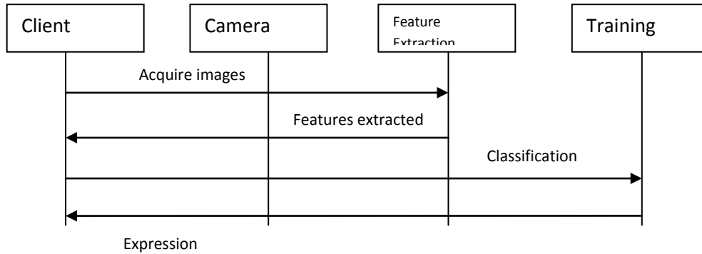
Figure 3.7: Sequence diagram
