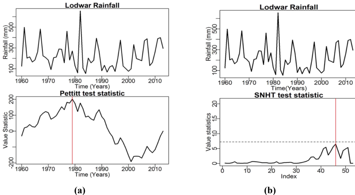
Figure 3: Test statistics of annual mean for (a) the Pettitt test and (b) the Standard Normal Homogeneity Test for Lodwar station.
